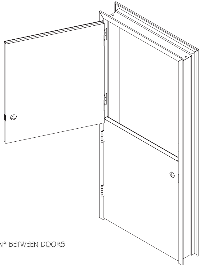
DUTCH DOOR SHOWN IN HOLLOW METAL FRAME
