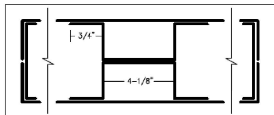
TOP VIEW OF SINGLE STIFFENER
