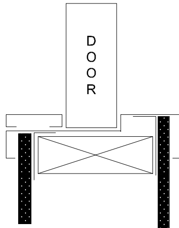
D-Strike Detail
