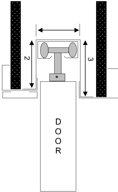
A - Head Detail
