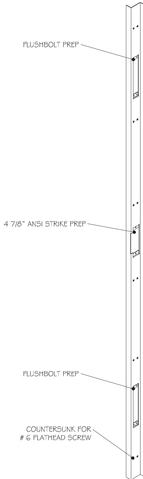
14 GAUGE STEEL "Z" ASTRAGAL
